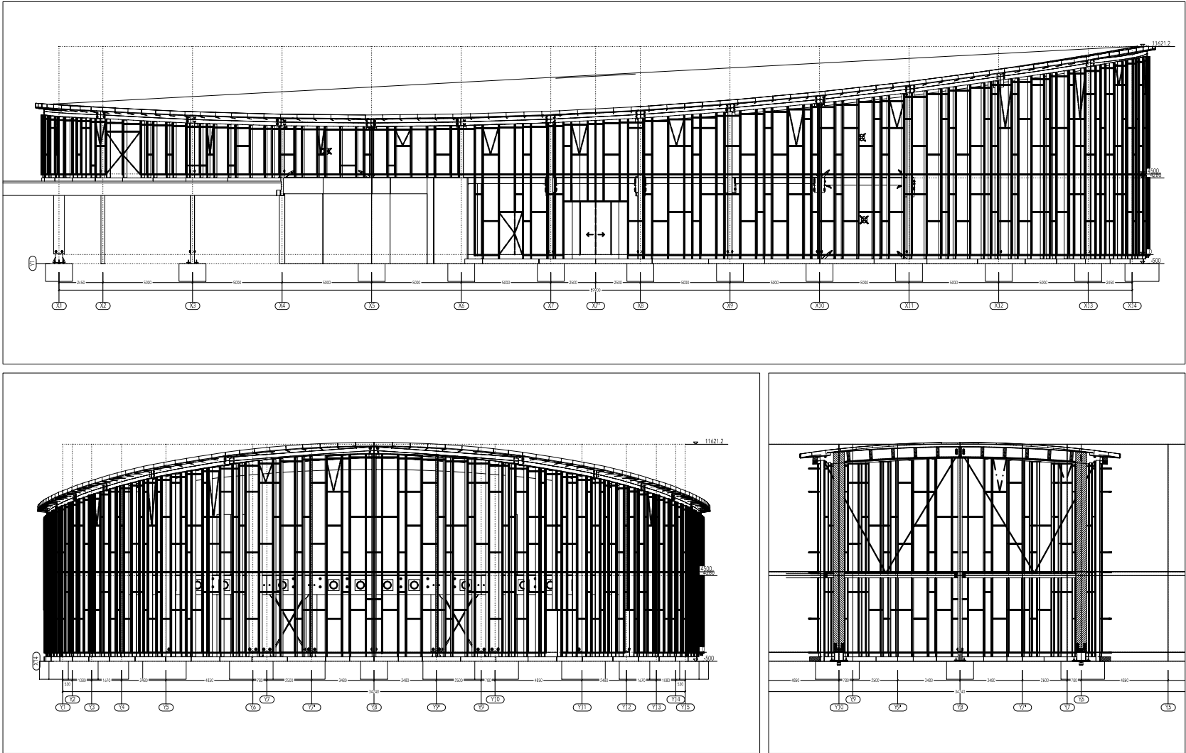
perspective drawing and internal view
